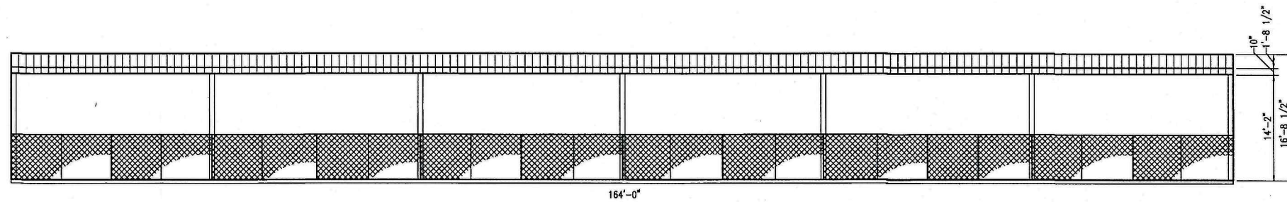
FRONT ELEVATION
