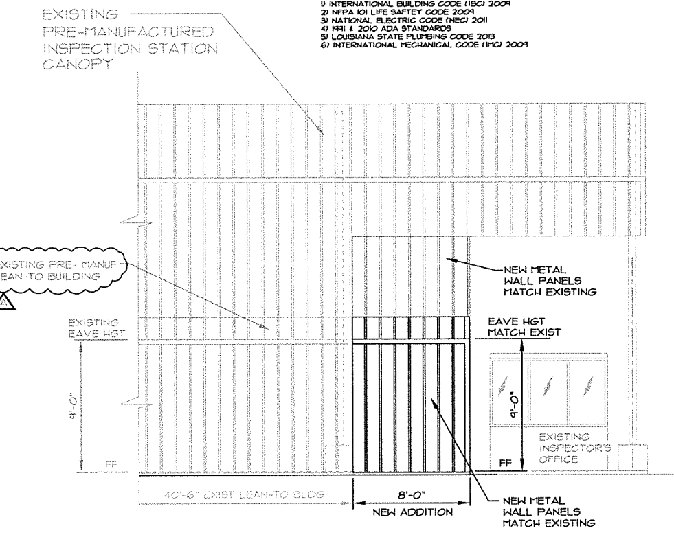
EAST ELEVATION "A-A" SCALE: 1/4"=1'-0"
