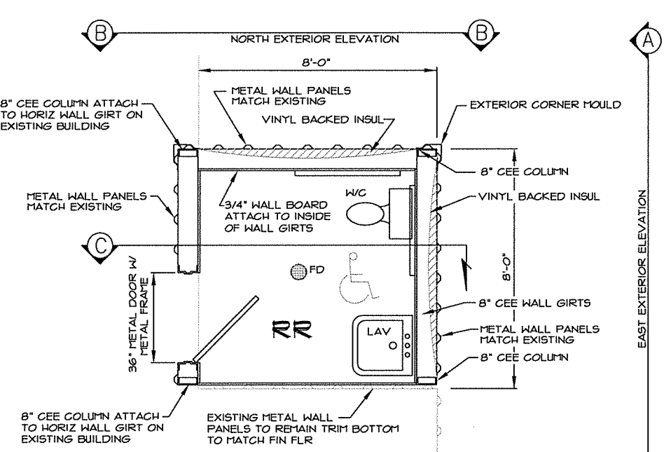
ADDITION FLOOR PLAN SCALE: 1/2"=1'-0"
