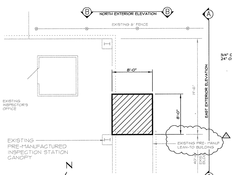
ENLARGED EXISTING FLOOR PLAN SCALE: 1/4"=1'-0"
