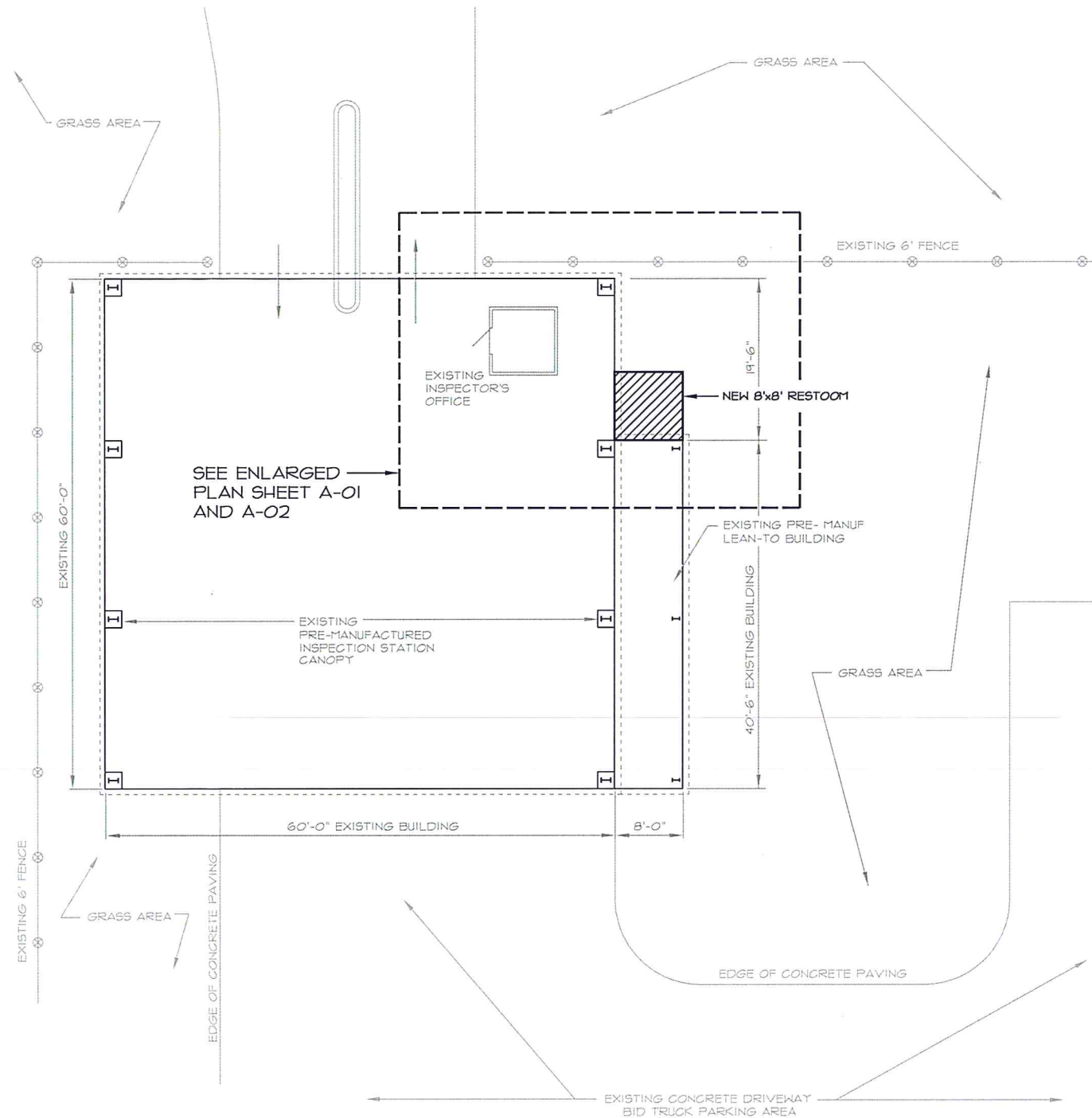
ENLARGED EXISTING SITE PLAN SCALE: 1"=50'-0"
