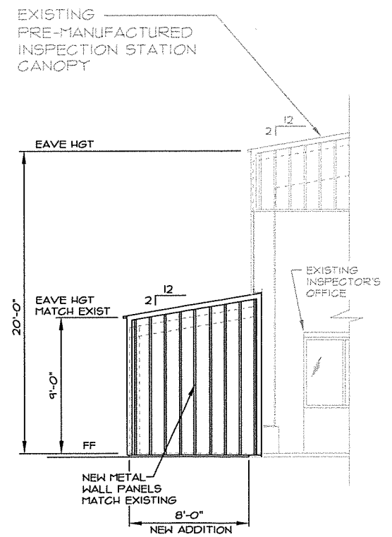
NORTH ELEVATION "B-B" SCALE: 1/4"=1'-0"
