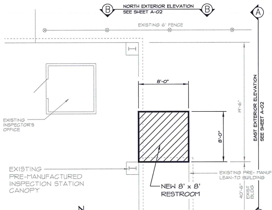
ENLARGED EXISTING FLOOR PLAN SCALE: 1/4"=1'-0"
