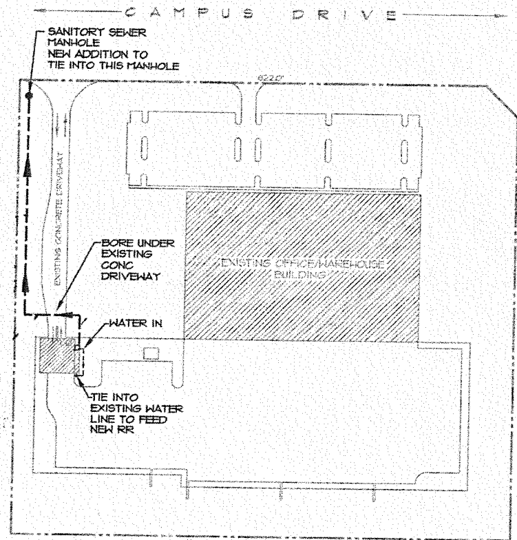
OVERALL PLUMBING SEWER SITE PLAN SCALE: 1"=100'-0"
