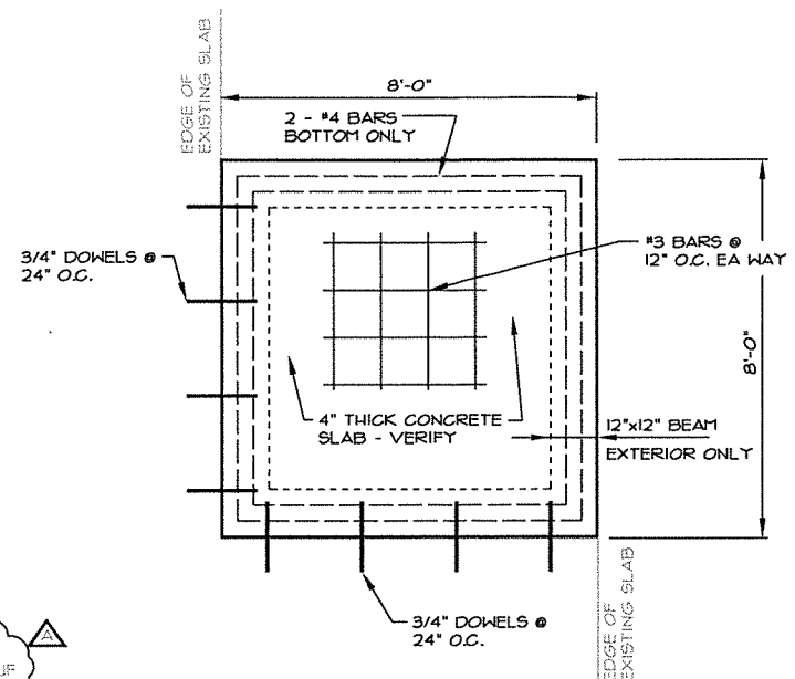
ADDITION FOUNDATION PLAN SCALE: 1/2"=1'-0"
